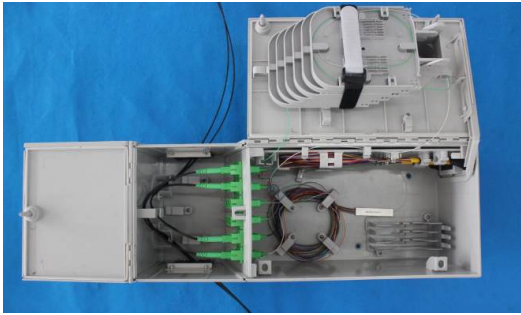
Opened MOTB-DG03 termination box
